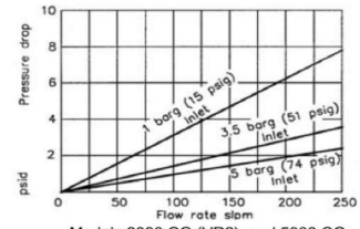
Models 3000 CG (VR2) and 5000 CG
