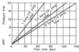
Models 1200 CG and 3000 CG (VR4)
